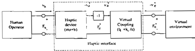
Fig.2 Two-port network of an impedance display haptic interface with a virtual coupling.
