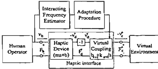
Figure 4. Schematic Diagram of a Haptic System with an Adaptive Virtual Coupling
