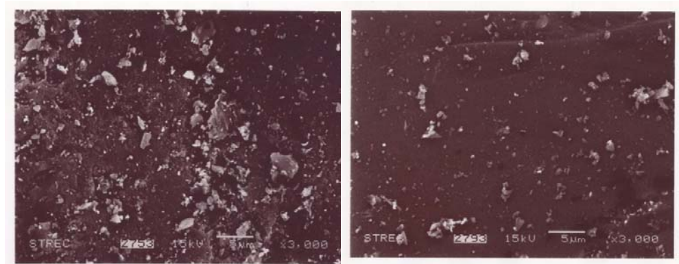
Pd-Ac/SiO 2
