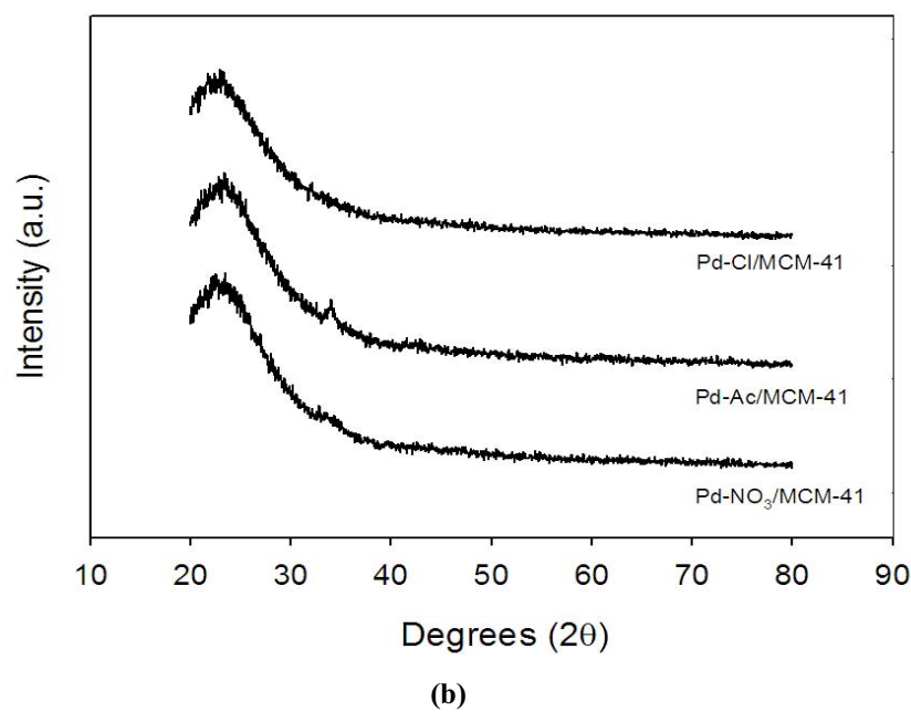
Figure 1 XRD patterns of various supported Pd catalysts prepared from different Pd precursors: (a) SiO 2 -supported Pd catalysts, (b) MCM-41-supported Pd catalysts (after calcinations at 500°C for 2 h).
