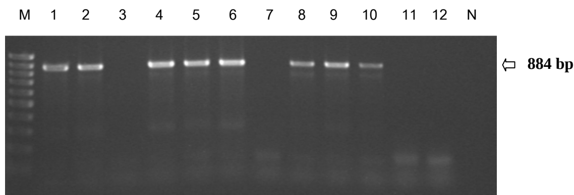
Figure 1. Detection of the invA gene homologue in Leptospira by PCR using Flank invA 5' and Flank invA 3' as primers. Lanes: 1, serovar Lai; 2, Bangkok; 3, Javanica; 4, Rachmati; 5, Bratislava; 6, Autumnalis; 7, Saigon; 8, Icterohaemorrhagiae; 9, Pyrogenes; 10, Bataviae; 11, Sejroe; 12, Patoc; M, 100-base pairs (bp) molecular weight marker; N, negative control without DNA
