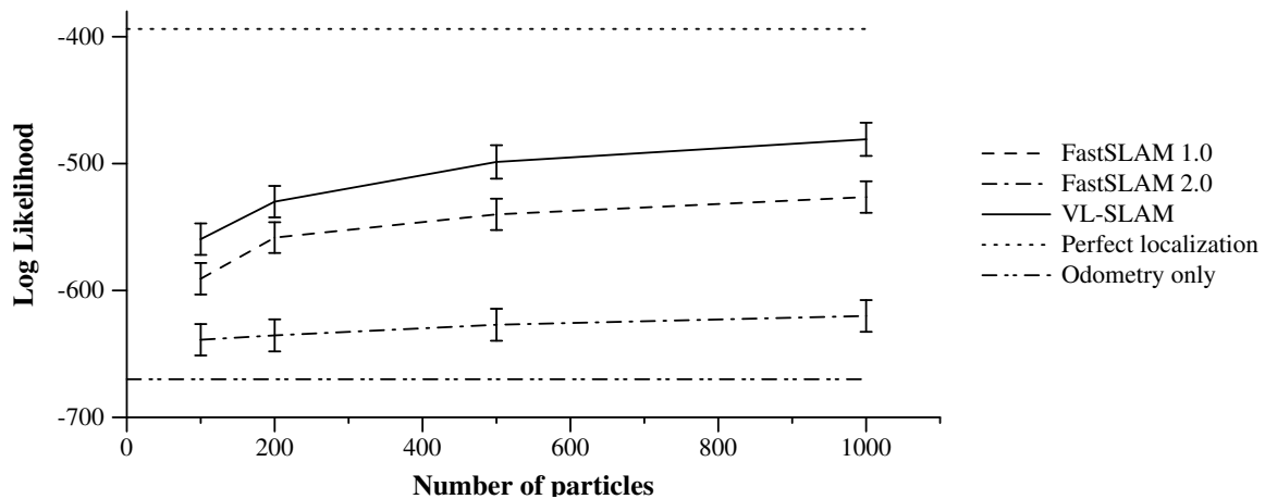
Fig. 2. Log likelihood of line observations according to the best particle's sampled robot position and map, averaged over 320 sets of observations.
