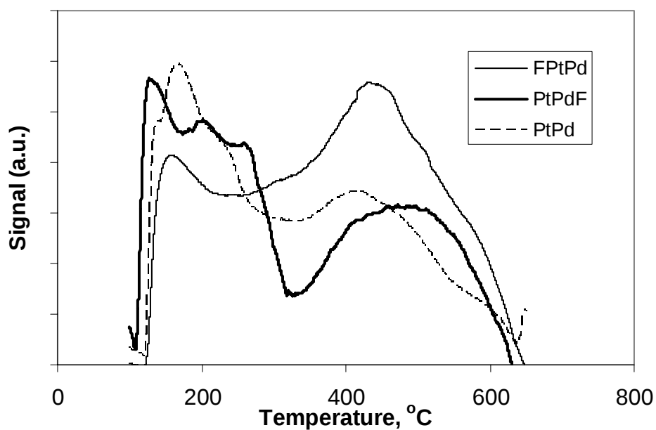
Fig. 3. TPD profiles of ammonia desorption of PtPd/Al 2 O 3 , PtPdF/Al 2 O 3 and FPtPd/Al 2 O 3 catalysts
