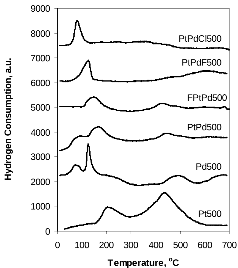
Fig. 2. Temperature Programmed Reduction of mono- and bi-metallic Pt-Pd catalysts calcined at 500°C prepared with and without F and Cl.
