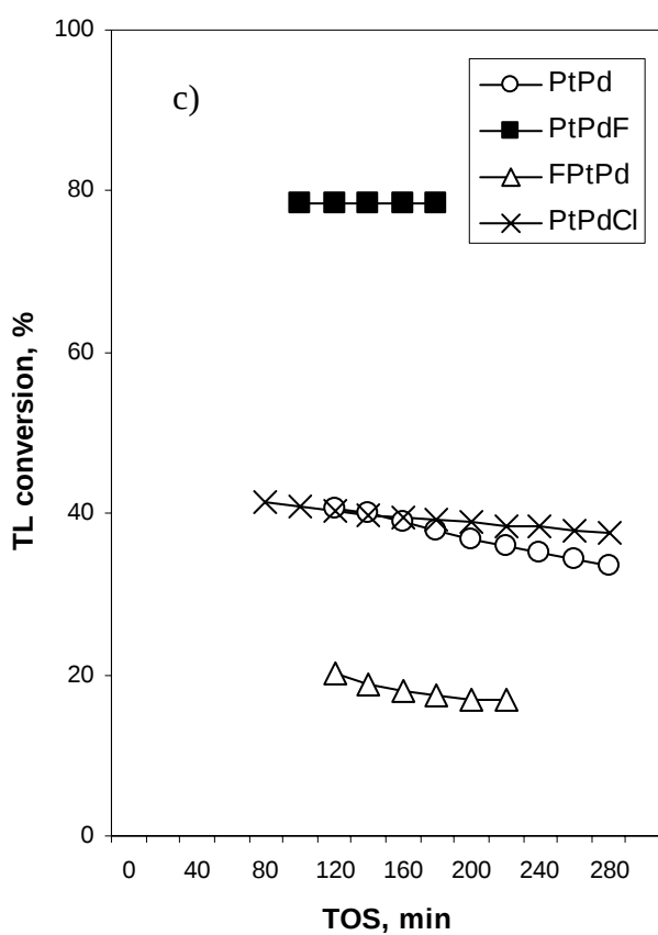
Fig. 4. Tetralin conversion as a function of time-on-stream in the absence of the S-compound. Reaction conditions: 300°C and 500 psi, H_2/HC = 11 , LHSV = 100 \text{ h}^{-1} . a) Pt/ Al_2O_3 catalysts; b) Pd/ Al_2O_3 catalysts; and, c) PtPd/ Al_2O_3 catalysts.
