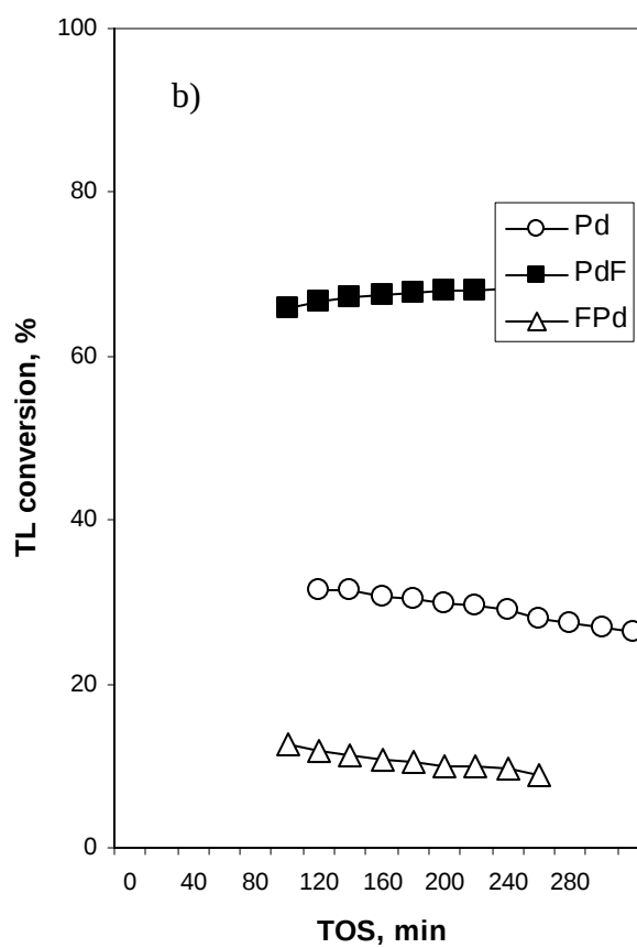
Fig. 4. Tetralin conversion as a function of time-on-stream in the absence of the S-compound. Reaction conditions: 300°C and 500 psi, H_2/HC = 11 , LHSV = 100 \text{ h}^{-1} . a) Pt/ Al_2O_3 catalysts; b) Pd/ Al_2O_3 catalysts; and, c) PtPd/ Al_2O_3 catalysts.
