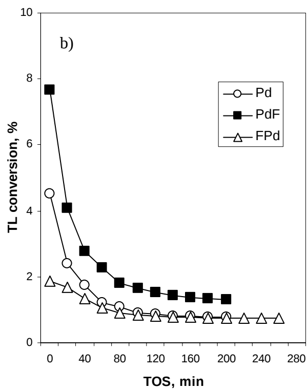
Fig. 6. Tetralin conversion as a function of time-on-stream in the presence of 350 ppm S. Reaction conditions: 300°C and 500 psi, H_2/HC = 11 , LHSV = 100\ h^{-1} . a) Pt/ Al_2O_3 catalysts; b) Pd/ Al_2O_3 catalysts; and, c) PtPd/ Al_2O_3 catalysts.
