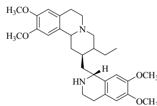
Emetine (1)
