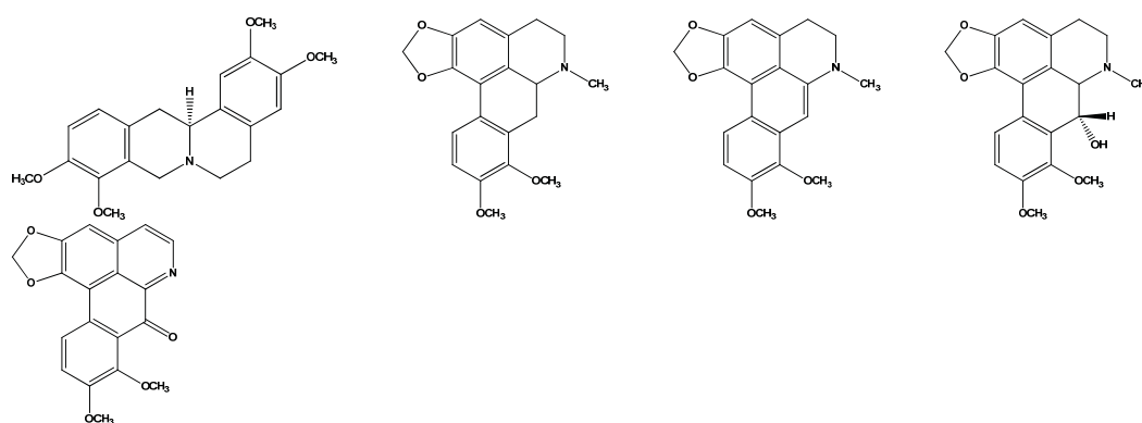
(-)-Tetrahydropalmatine (1) (-)-Crebanine (2) Dehydrocrebanine (3) (-)-Sukhodianine (4) Oxocrebanine (5)
