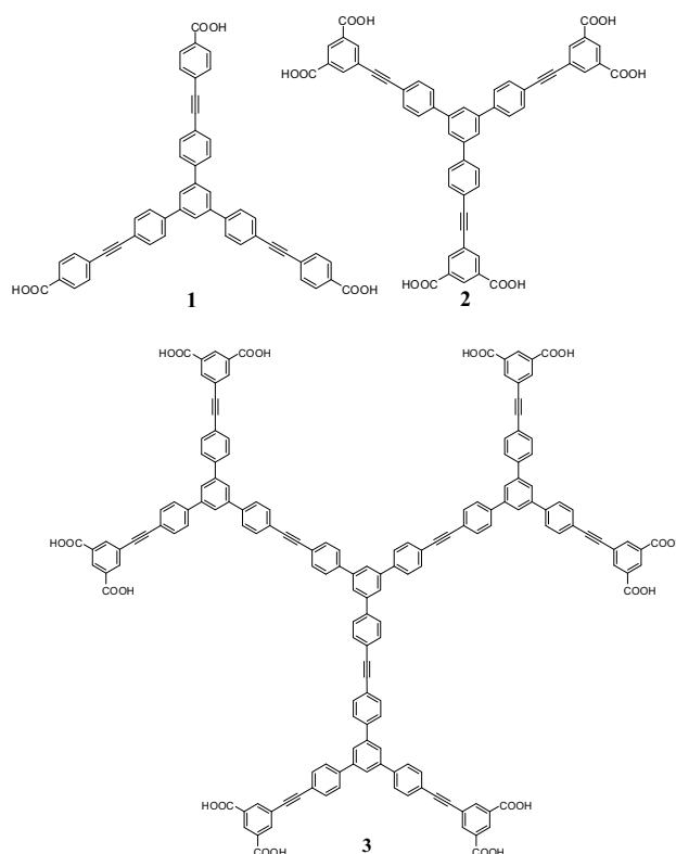
Figure1. Structures of dendritic fluorophores 1-3.
