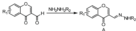
Scheme 1. Synthesis of chromone hydrazons A1- A13. Chromone derivatives with various hydrazines in ethanol. stir 2-4 hr., RT.
