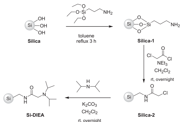
Scheme 1. Synthesis of Si-DIEA
