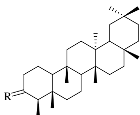
(1) friedelin, R= O (2) epifriedelanol, R=3 \alpha -OH, 3 \beta -H (3) friedelanol, R=3 \beta -OH, 3 \alpha -H
