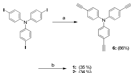
Scheme 2. Reagents and conditions: (a) i. trimethylsilyl acetylene, \text{PdCl}_2(\text{PPh}_3)_2 , CuI, \text{NEt}_3 ; ii. \text{K}_2\text{CO}_3 , \text{CH}_2\text{Cl}_2 , MeOH (1:1); (b) i. 5a or 5c , \text{PdCl}_2(\text{PPh}_3)_2 , CuI, DBU, PhMe; ii. KOH, THF, MeOH.
