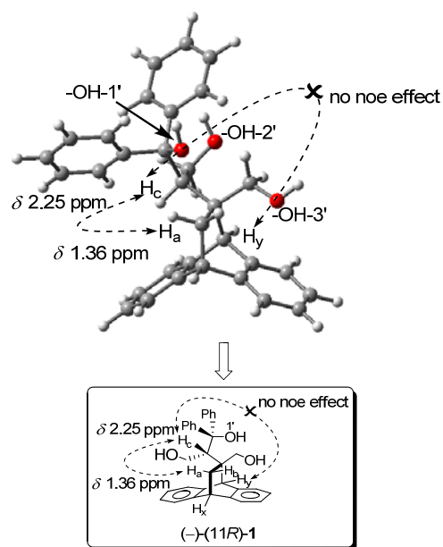
Figure 3. 3D structural conformation of TADDOL–anthracene adduct (–)-(11 R )- 1 generated by MM2 force field calculations for energy minimization from modeling program ChemBio3D Ultra 11.0 and GaussView 3.09 program
