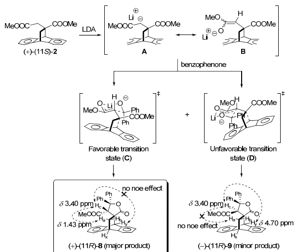
Scheme 2. Proposed mechanism of the adducts (+)-(11 R )- 8 and (–)-(11 R )- 9 .
