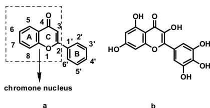
Figure 3. (a) General flavonoid structure. (b) Myricetin structure.
