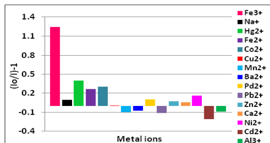
Figure 2. Fluorescence responses of 1 (4 \mu\text{M} ) to various metal ions (400 \mu\text{M} ) in phosphate buffer (50 mM, pH 8.0).
