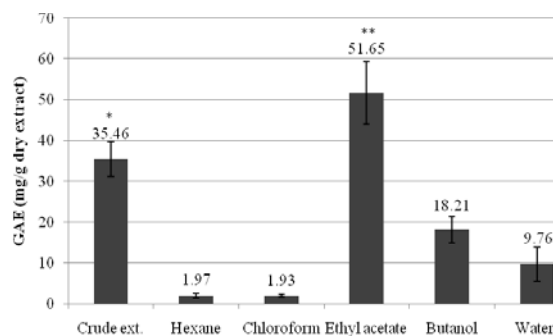
Figure 1. GAE value of P. emblica fractions
