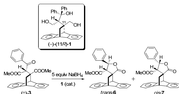
Figure 2. The reduction of the \beta -keto diester [( \pm )- 3 ] using TADDOL–anthracene 1 catalyst
