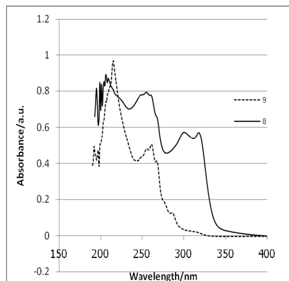
Figure 2. Absorbance spectra of 8 and 9
