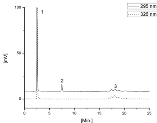
รูปที่ 10.2 Chromatogram of standards at wavelength of 295 and 326 nm using ACE C18-AR column in mobile phase as methanol : acetic acid (99.5:0.5) at flow rate 1.2 ml/min. Peaks: (1) ferulic acid (2) \alpha -tocopherol (3) \gamma -oryzanol
