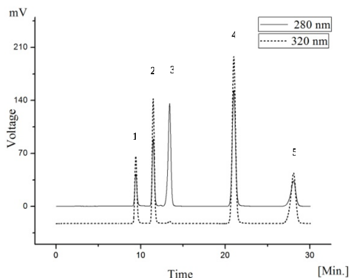
รูปที่ 10.1 Chromatogram of standards at wavelength of 280 and 320 nm using ACE C18-AR column in mobile phase as 2% (v/v) acetic acid in water – methanol 82:18 (v/v) at flow rate 1.2 ml/min. Peaks : (1) chlorogenic acid; (2) caffeic acid; (3) syringic acid; (4) p -Coumaric acid; (5) ferulic acid.
