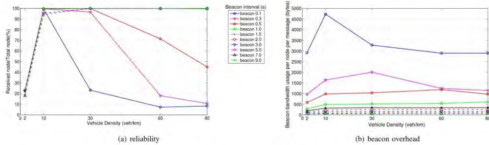
Fig. 1: Simulation results in Urban scenarios (using constant beaconing rate)
