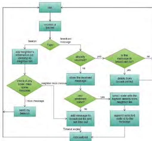
Figure 1. Flowchart showing how DECA works
