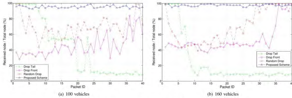
Fig. 5: Reliability with buffer size 5 packets
