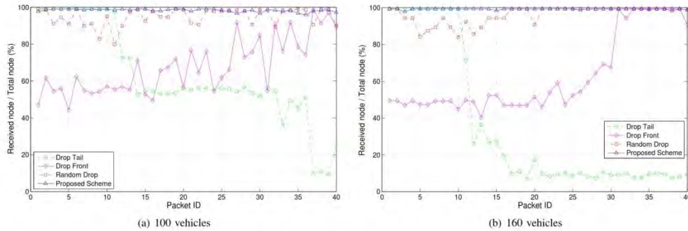
Fig. 6: Reliability with buffer size 10 packets
