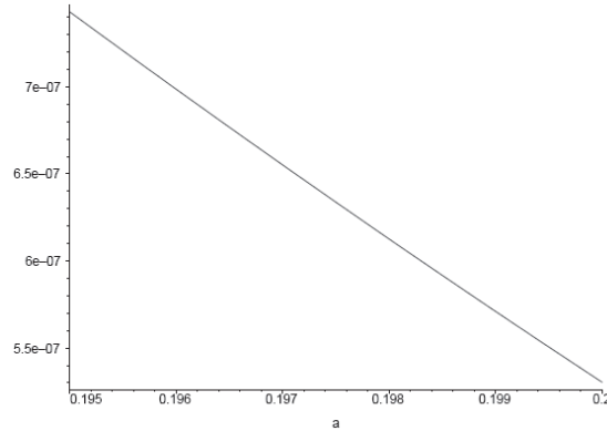
FIGURE 5. The bounds on the greybody factors as a function of a with \zeta \cong 1, Q \cong 0.21, \ell = 2, m = 1 and M \cong 0.3 .
