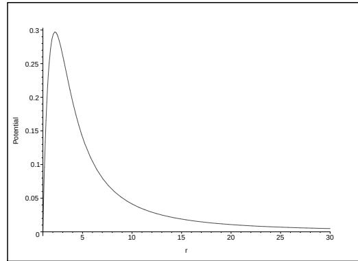
Figure 1: The Myers-Perry potential for n = 1 .
