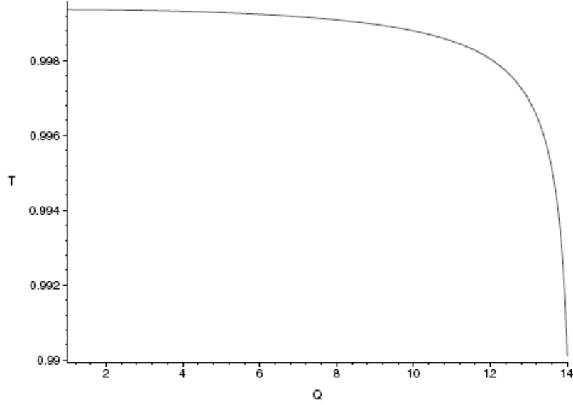
Figure 7. Dependence of the bound on the greybody factor on the charge of the dilatonic black holes in (3 + 1) dimensions.
