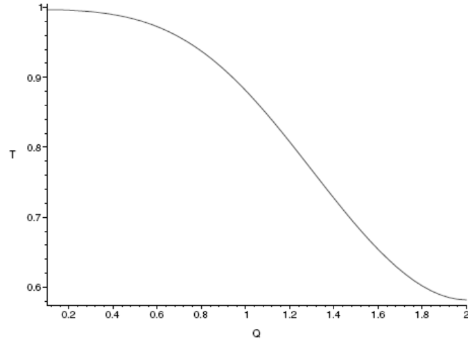
Figure 4. Dependence of the bound on the greybody factor on the charge of the dilatonic black holes in (2 + 1) dimensions.
