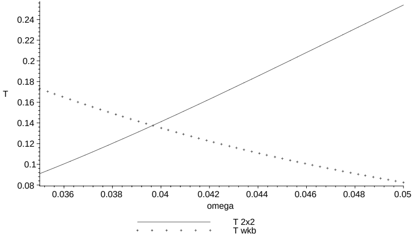
Fig. 3. Comparison of the greybody factor bound of the RN black hole from the 2 \times 2 transfer matrix and the WKB approximation.
