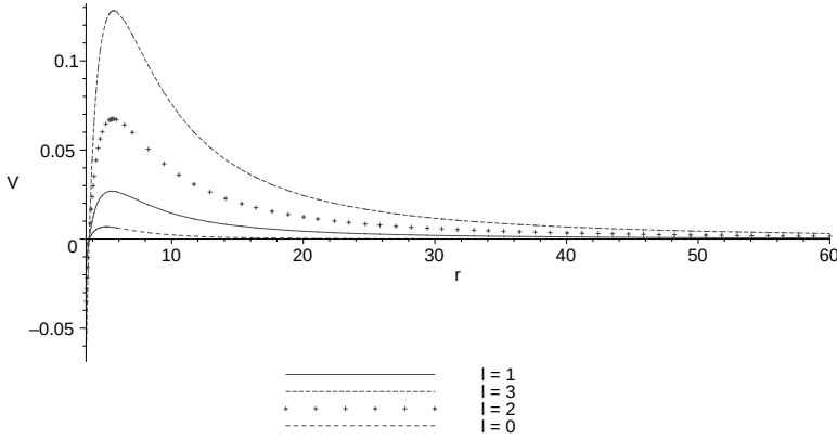
Fig. 1. The RN potential with Q = 1 and M = 2 in different angular momenta.
