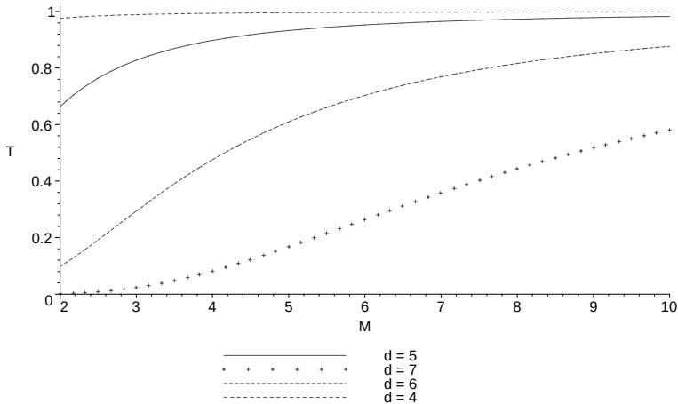
Fig. 6. Dependence of the greybody factor bound on the black hole mass in various dimensions.
