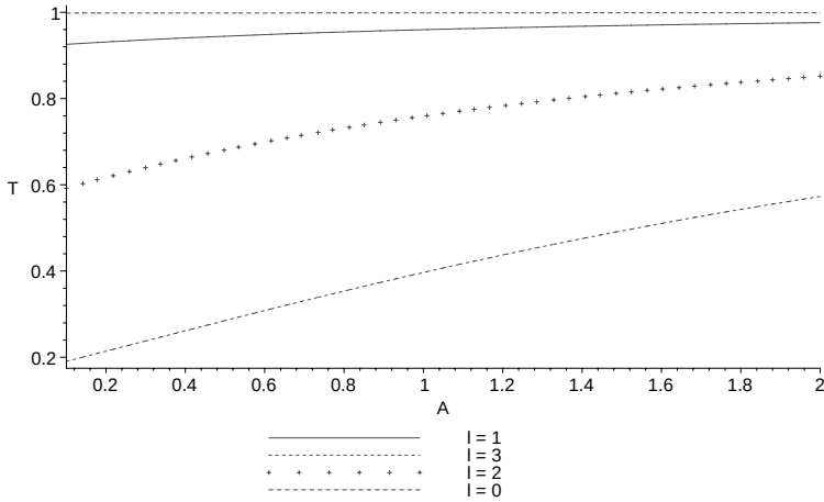
Fig. 2. Dependence of the bound of the greybody factor on the RN black hole charges in different angular momenta.
