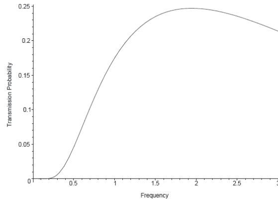
FIGURE 1. The bounds on the greybody factors as a function of \zeta with a \cong 2, Q \cong 2, \ell = 2, m = 01 and M \cong 3 .
