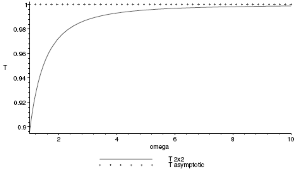
Figure 2. Comparison of the bound on the greybody factor and the asymptotic greybody factor.
