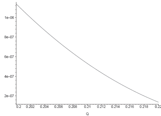
FIGURE 6. The bounds on the greybody factors as a function of Q with \zeta \cong 1, a \cong 0.2, \ell = 2, m = 1 and M \cong 0.3 .
