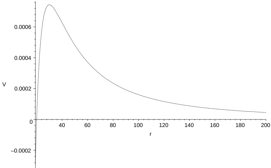
Fig. 11. The (3 + 1) charged dilatonic potential with l = 1 , Q = 1 and M = 10 .
