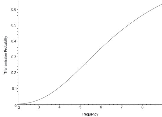
FIGURE 4. The bounds on the greybody factors as a function of \zeta with a \cong 0.2, Q \cong 0.21, \ell = 2, m = 1 and M \cong 0.3 .
