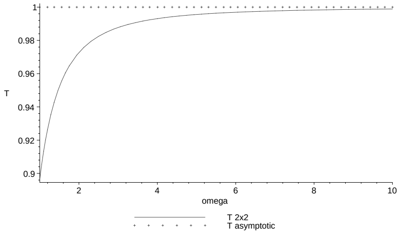
Fig. 4. Comparison of the greybody factor bound of the RN black hole from the 2 \times 2 transfer matrix and the asymptotic result.
