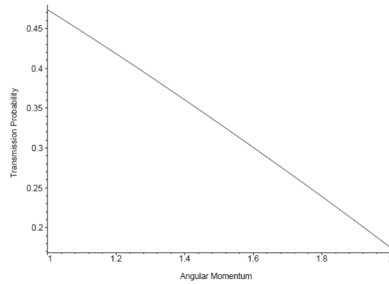
FIGURE 2. The bounds on the greybody factors as a function of a with \zeta \cong 1, Q \cong 2, \ell = 2, m = 01 and M \cong 3 .
