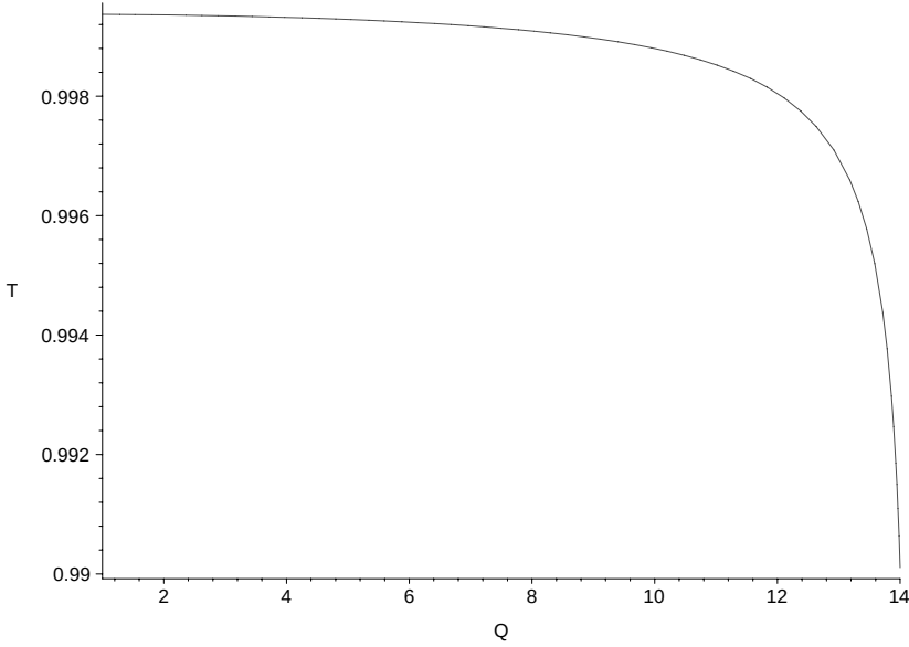
Fig. 12. Dependence of the greybody factor bound on the charges for the charged dilatonic black holes in (3 + 1) dimensions.
