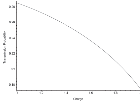
FIGURE 3. The bounds on the greybody factors as a function of Q with \zeta \cong 1, a \cong 2, \ell = 2, m = 0 and M \cong 3 .
