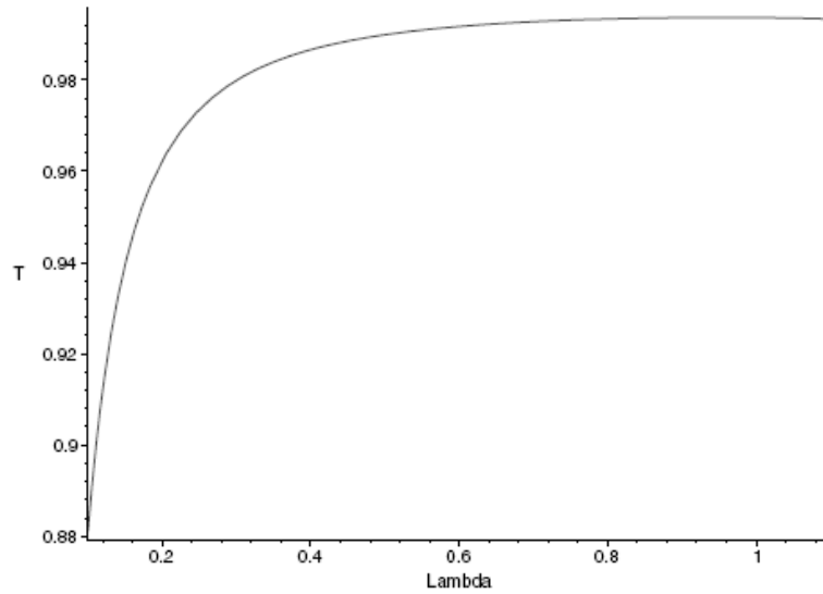
Figure 5. Dependence of the bound on the greybody factor on the cosmological constant for the charged dilatonic black holes in (2 + 1) dimensions.
