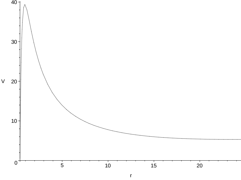
Fig. 7. The (2 + 1) charged dilatonic potential with m = 1 , \Lambda = 0.1 , Q = 1 and M = 10 .
