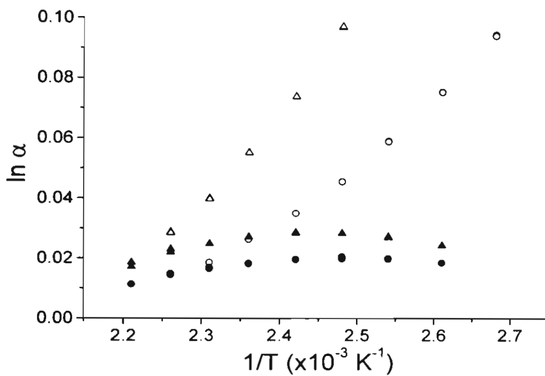
Fig. 5. \ln \alpha versus 1/T plots of alcohols 1 ( \circ ), 14 ( \bullet ), 16 ( \blacktriangle ), and 19 ( \triangle ) obtained with a chiral BSMe column
