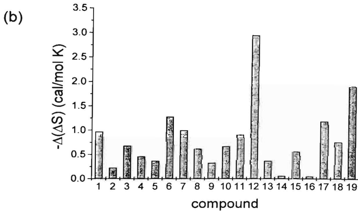
Fig. 4. Difference in enthalpy (a) and entropy (b) values for enantiomeric pair of alcohols on a chiral BSMe column
