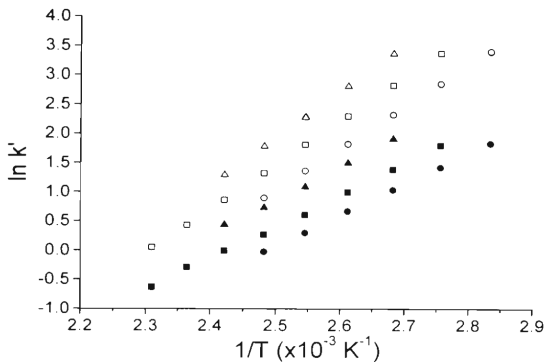
Fig. 2. \ln k' versus 1/T plots of alcohols 1-3 obtained with a nonchiral OV-1701 column (solid symbols) and of the more retained enantiomer of alcohols 1-3 obtained with a chiral BSMe column (open symbols): compounds 1 (■/□), 2 (●/○) and 3 (▲/△)
