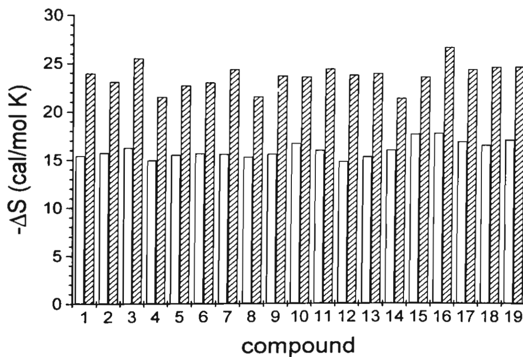
Fig. 3. Enthalpy (a) and entropy (b) values of all alcohols on a nonchiral OV-1701 column (solid color) and of more retained enantiomers on a chiral BSMe column (hatch)
