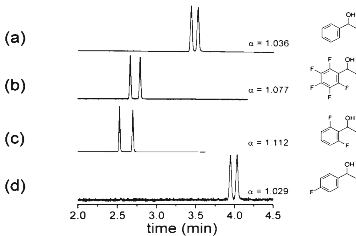
Fig. 6. Enantiomer separation of alcohols 1 (a), 19 (b), 12 (c), and 7 (d) on a BSMe column at 140 °C isothermal
