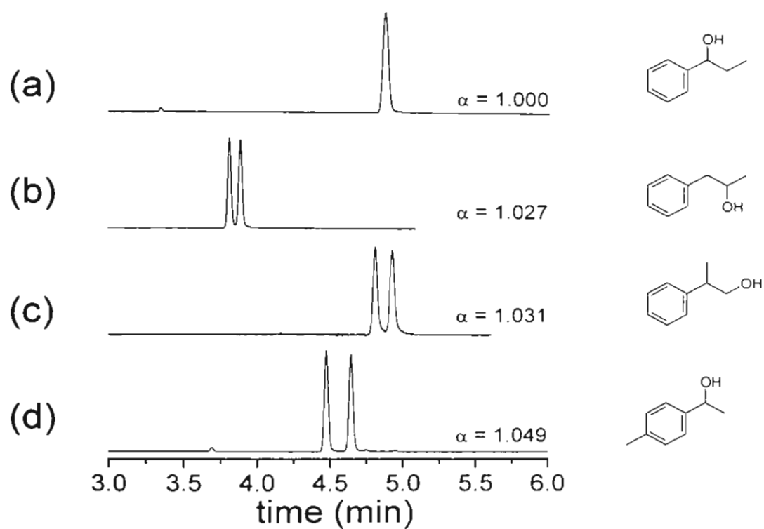
Fig. 7. Enantiomer separation of alcohol isomers 3 (a), 4 (b), 5 (c), and 6 (d) on a BSMe column at 140 °C isothermal
