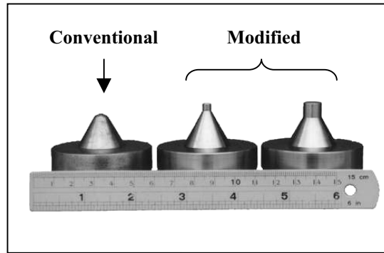
Figure 1 Conventional and modified loading points.
