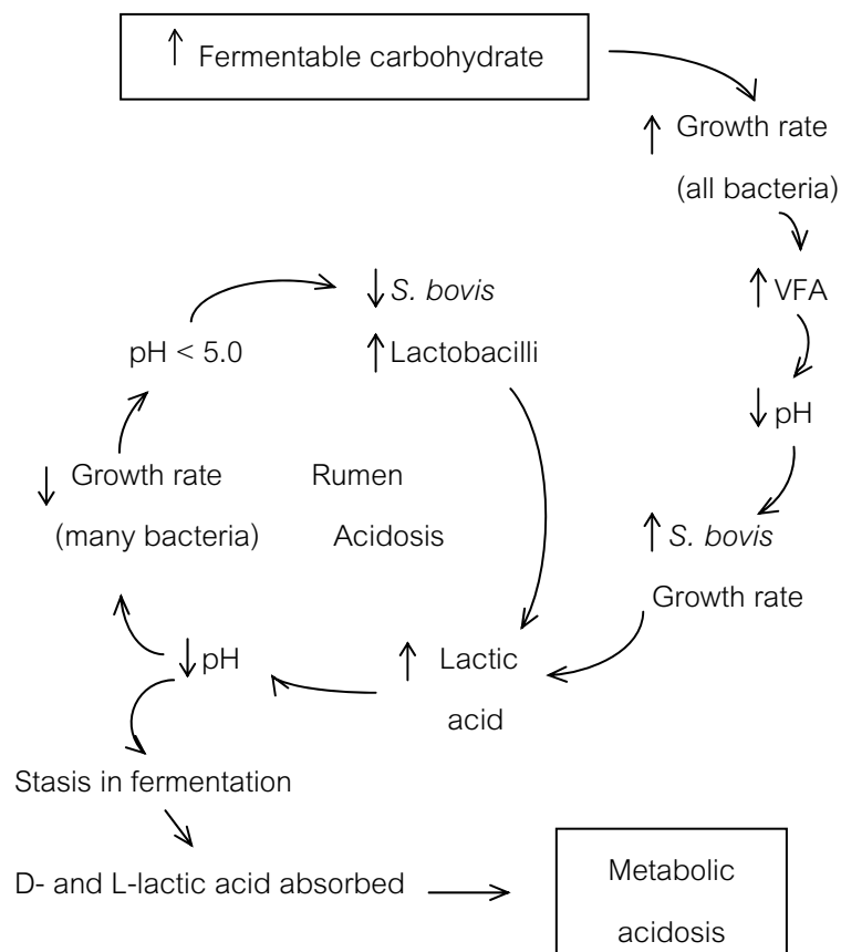
Figure 1 Sequence of events associated with the induction of acute ruminal lactic acidosis. (Nocek, 1997)
