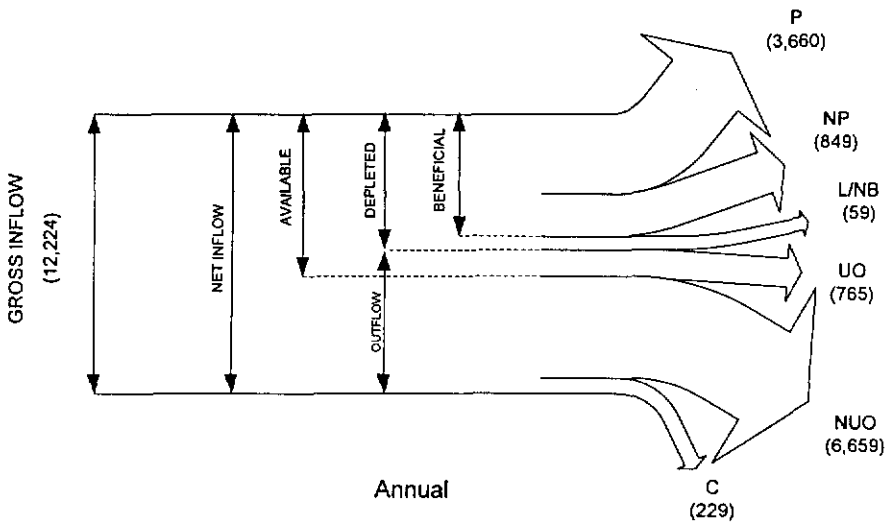
• Figure 28 Water Accounting Diagram of the Main Bang Pakong + Talat Sub Basins in Wet Year (1995)
