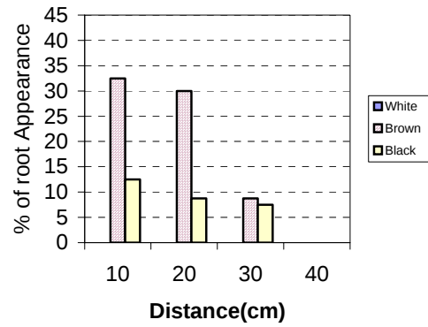
Root types distribution of sugarcane in distance (16-8-8)
