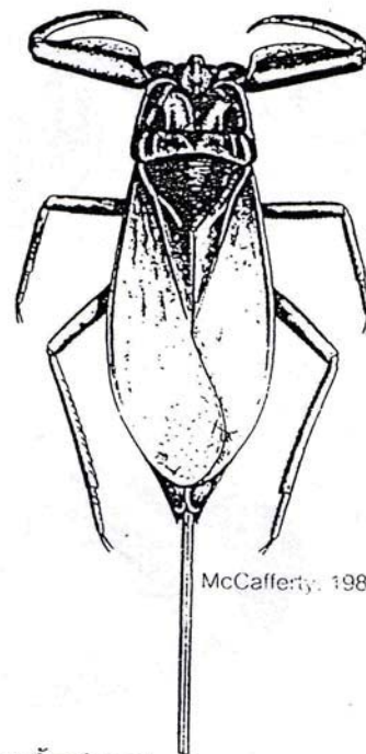
McCafferty, 1981
