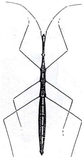
McCafferty, 1981
