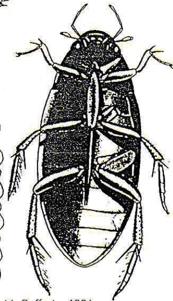
McCafferty, 1981
