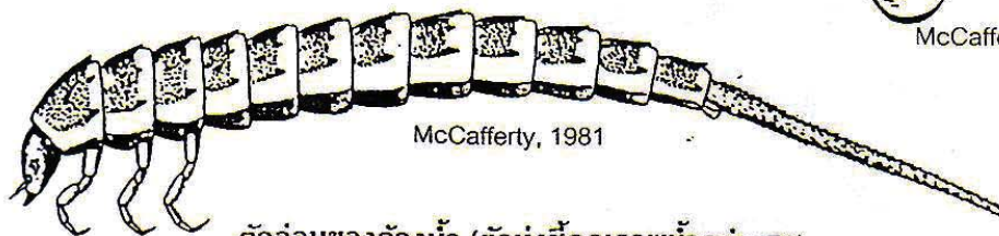
McCafferty, 1981
