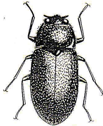
McCafferty, 1981
