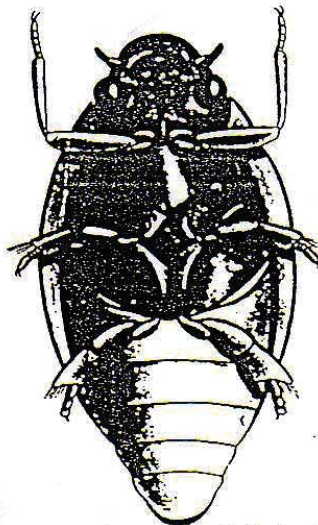
McCafferty, 1981
