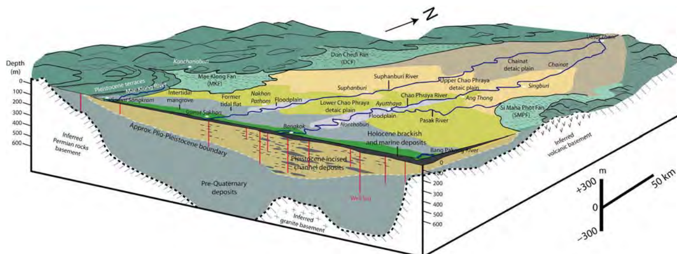
Fig. 12.6. Three-dimensional diagram of the Lower Central Plain showing distribution of landforms and Quaternary deposits (modified from Japan International Cooperation Agency 1995).
