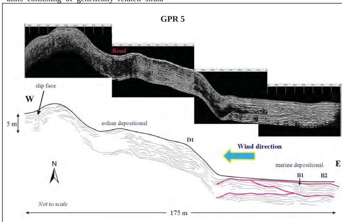
Figure 3. GPR 5 was conducted along – transects oriented parallel to the dune’s downwind axis. The characteristics of marine sediment are beach ridge (unit B1) generally dip seaward and littoral deposit (unit B2) horizontal layer. Slip-faces of dune represent the probable direction of wind blown from the east to the west.
