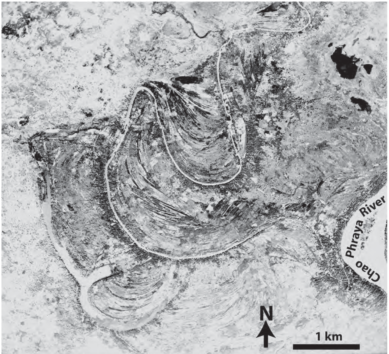
Fig. 12.5. Three meander belts of the Chao Phraya River, showing the avulsion plain that contains meander scars, oxbow lakes and swale and swell patterns within point bar deposits (from Tultaveewat et al. 2008).
