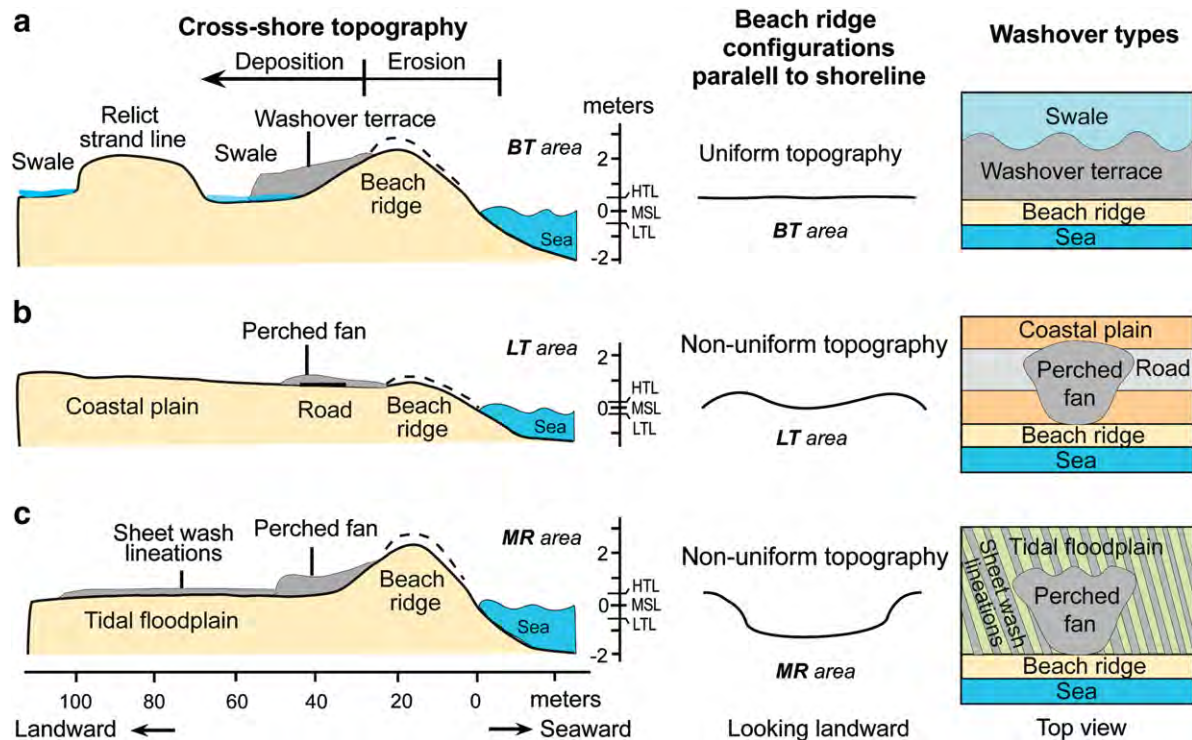
Fig. 11. Cross-shore topography and beach ridge configuration from three areas that control the preservation type and sedimentary characteristics of washover deposits. (a) A large swale behind the beach and uniform beach ridge configuration result in a washover terrace deposit at BT. (b) A flat and high coastal plain topography behind beach with a non-uniform beach ridge configuration results in perched fan deposits at LT. (c) The low-lying tidal floodplain behind the beach barrier associated with a non-uniform beach ridge configuration resulting in sheetwash lineations and perched fan deposition at MR. Beach ridge configurations (looking from seaward to landward) and washover preservation types (looking from top view). Cross-shore profile at BT is made from survey data, whereas BT and LT profiles are from qualitative sketch.
