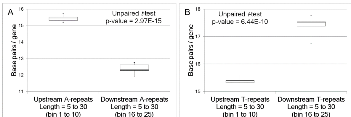
Figure 3. Box plots of numbers of A- and T-repeats in bins 1–10 and bins 16–25. The unpaired t -test was used to compare the mean difference between upstream repeats (bins 1–10) and downstream repeats (bins 16–25).
