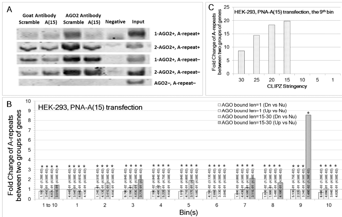
Figure 10. Inhibition of AGO binding to A-repeats. (A) PNA-A(15) reduced AGO2 binding to long A repeats. ChIP assays for AGO2-bound sequences were performed in HEK-293 cells transfected with control PNA (scramble) or test PNA-A(15) [A(15)] oligos. A control goat antibody was used as the negative control for the AGO2-bound sequences. Distilled water and sonicated DNA input were used as negative and positive controls for PCR, respectively. Reductions of AGO2 binding to A repeats in the presence of PNA-A(15) were demonstrated at AGO2 bound A-repeats using two AGO2+and A-repeat+PCR primer sets (AGO2+, A-repeat+). No reduction of AGO2 binding to unique DNA sequences in the presence of PNA-A(15) was observed using two AGO2+and A-repeat-PCR primer sets (AGO2+, A-repeat-). No AGO2 binding to AGO2-negative locations was detected (AGO2-, A-repeat-). (B) HEK-293 PNA-A(15) transfection. The fold changes in the number of A-repeats between Dn/Up and Nu, which denote down/upregulated and non-regulated (neutral) genes, respectively. The horizontal axis indicates the bin location. The Ago-bound length is the length of the repeat that is actually bound by Ago proteins, not the entire repeat length. The first column shows the sums of bins 1–10. The two numbers ' p ( q )' in each bar are the P -value and q -value, respectively. Single stars indicate low confidence (FDR or q \leq 0.05 ), and double stars indicate high confidence (FDR or q \leq 0.01 ). (C) The fold changes in the number of A-repeats between upregulated (Up) and non-regulated (Nu) genes in the ninth bin of HEK-293 PNA-A(15) transfected cells. The horizontal axis is the stringency threshold; lower numbers correspond to greater stringency. AGO-bound sequences that can be aligned to a number of genomic loci greater than the stringency threshold were excluded from the fold-change calculation.
