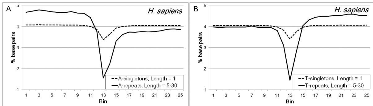
Figure 2. Comparisons between A/T-singletons (length=1) and A/T-repeats (length=5–30 bp) around TSS in the whole genome. The horizontal axis consists of 25 bins. Each bin covers 800 bp, with 10,000 bp upstream and 10,000 bp downstream of TSS in total. The TSS is centered in the 13 th bin. The vertical axis represents the number of base pairs normalized to the percentage of all nucleotides. (A) A-repeats. (B) T-repeats.
