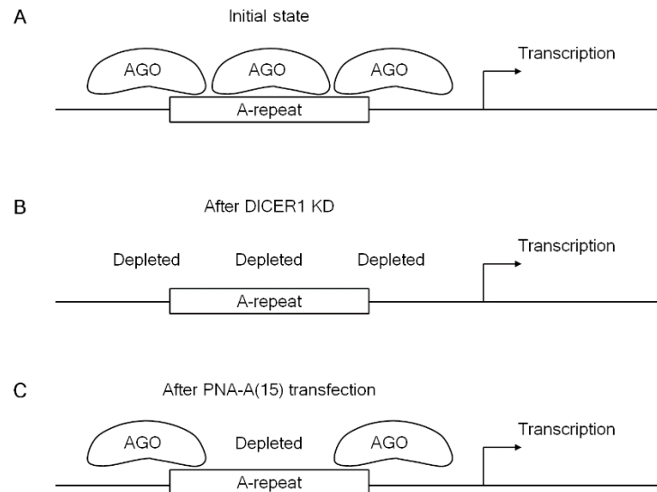
Figure 6. Expected results of DICER1 KD and PNA-A(15) transfection. (A) In the initial state, three Ago complexes bind upstream of the TSS. (B) DICER1 KD depletes all Ago binding, independent of target sequences. (C) PNA-A(15) transfection depletes only Ago complexes that bind to intact A(15).
