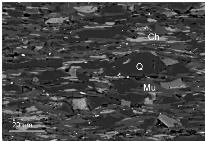
Fig. 1. Backscatter electron SEM image of La Fortelle slate. Polished section cut perpendicular to the foliation; foliation plane is horizontal. Dark is quartz (Q), medium gray is muscovite (Mu), light gray is chlorite (Ch), and white is pyrite and rutile.
