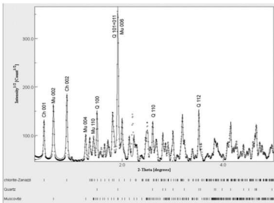
Fig. 4. X-ray diffraction pattern of slate with some peak identifications: Q is quartz, Mu is muscovite, and Ch is chlorite. This pattern is an azimuthal average over the diffraction
