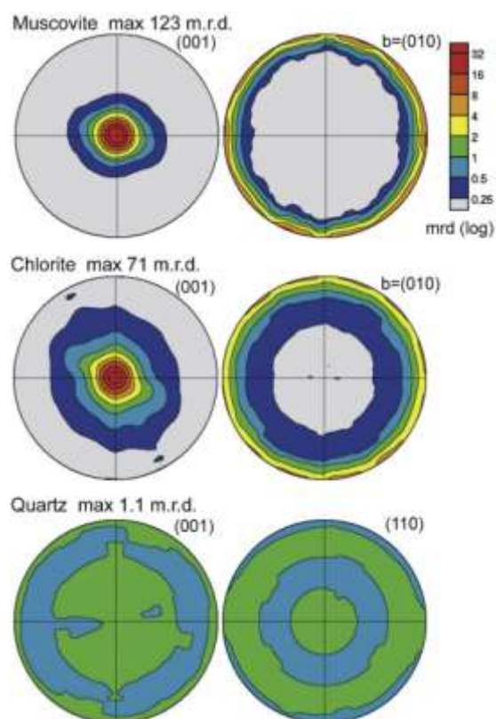
Fig. 5. Pole figures of muscovite, chlorite, and quartz on the foliation plane. Equal area projection, log scale for pole densities in multiples of random distribution (m.r.d.).
