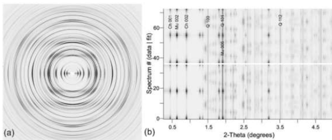
Fig. 3. (a) X-ray diffraction image. Foliation plane is vertical. (b) Stack of 36 diffraction spectra integrated over 10° sectors, corresponding to (a), bottom: experimental spectra, top: Rietveld refinement. Some diffraction peaks are indexed: Q is quartz, Mu is muscovite, and Ch is chlorite.
