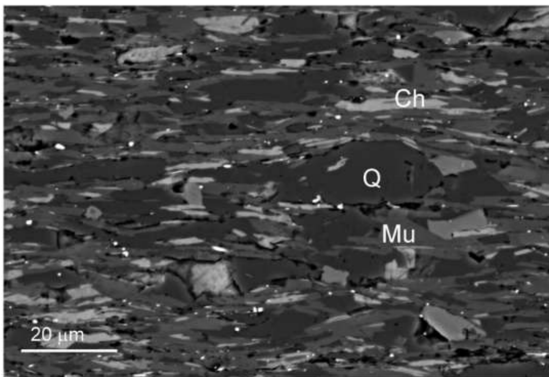
Fig. 1. Back-scattered electron SEM image of La Fortelle slate. Polished section cut perpendicular to the foliation; foliation plane is horizontal. Dark is quartz (Q), medium gray is muscovite (Mu), light gray is chlorite (Ch), and white is pyrite and rutile.
